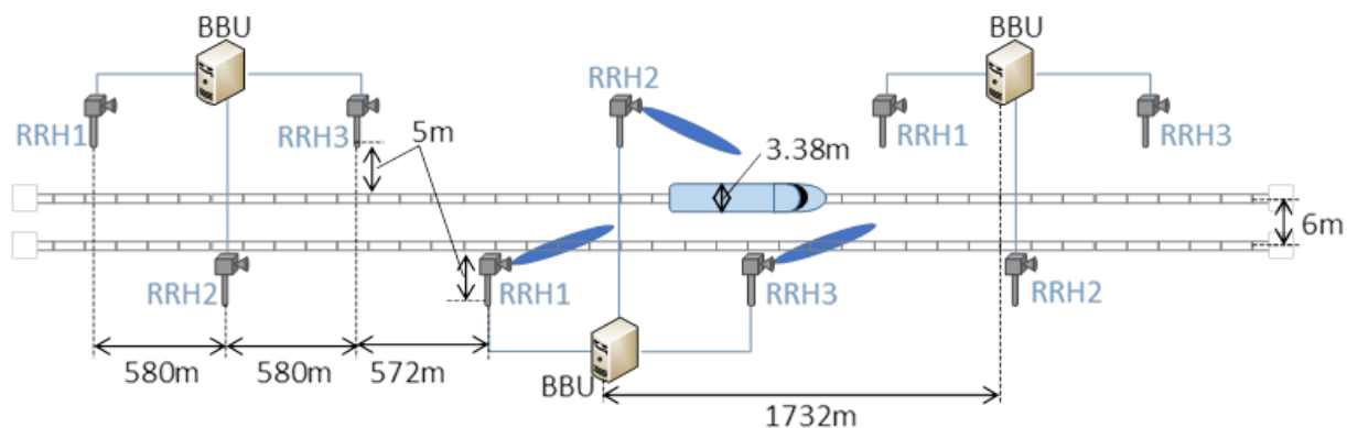
Figure 6.1.5-2: 30 GHz deployment
