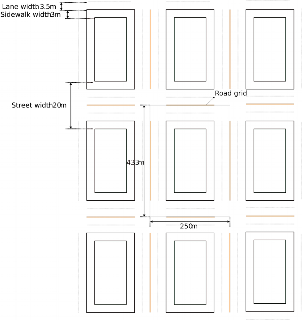
Figure 6.1.9-1: Road configuration for urban grid
