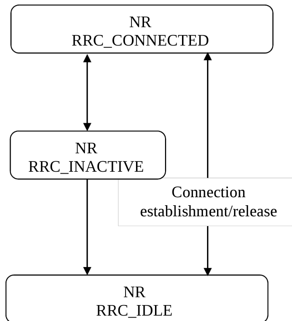
Figure 9.8.2-1: UE state machine and state transitions in NR
