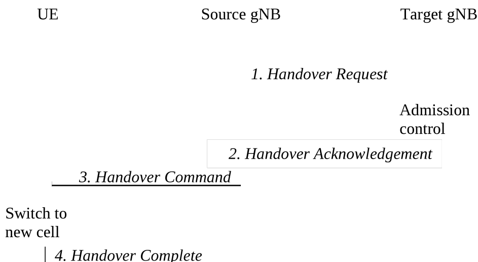
Figure 13.2.1.2-1: Inter-gNB handover procedures
