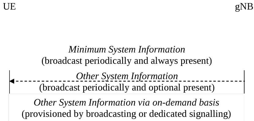
Figure 9.8.3-1: High level concept of on-demand SI provisioning
