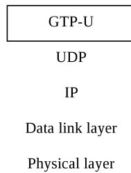
Figure 10.3.2.1.4-1: Xn Interface User Plane
