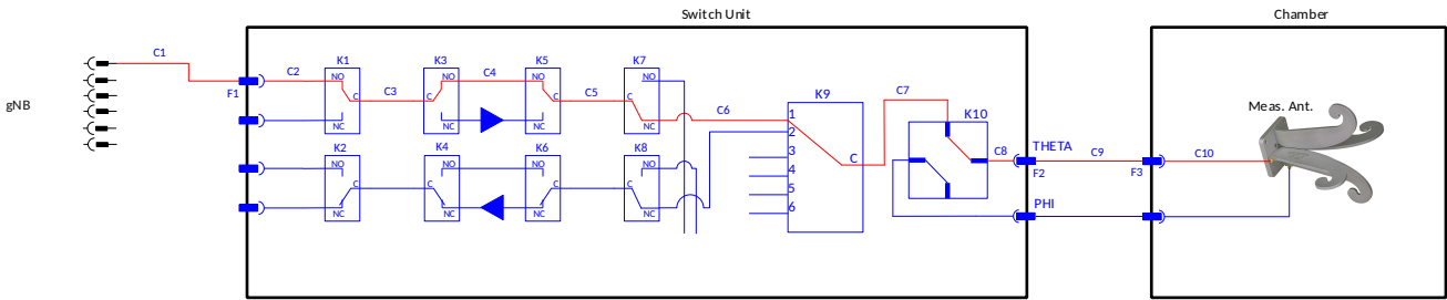
Figure B.2.1.4-3: Block Diagram of an EIRP/EIS test case with components from the gNB to the antenna (only portion of switch unit shown)
