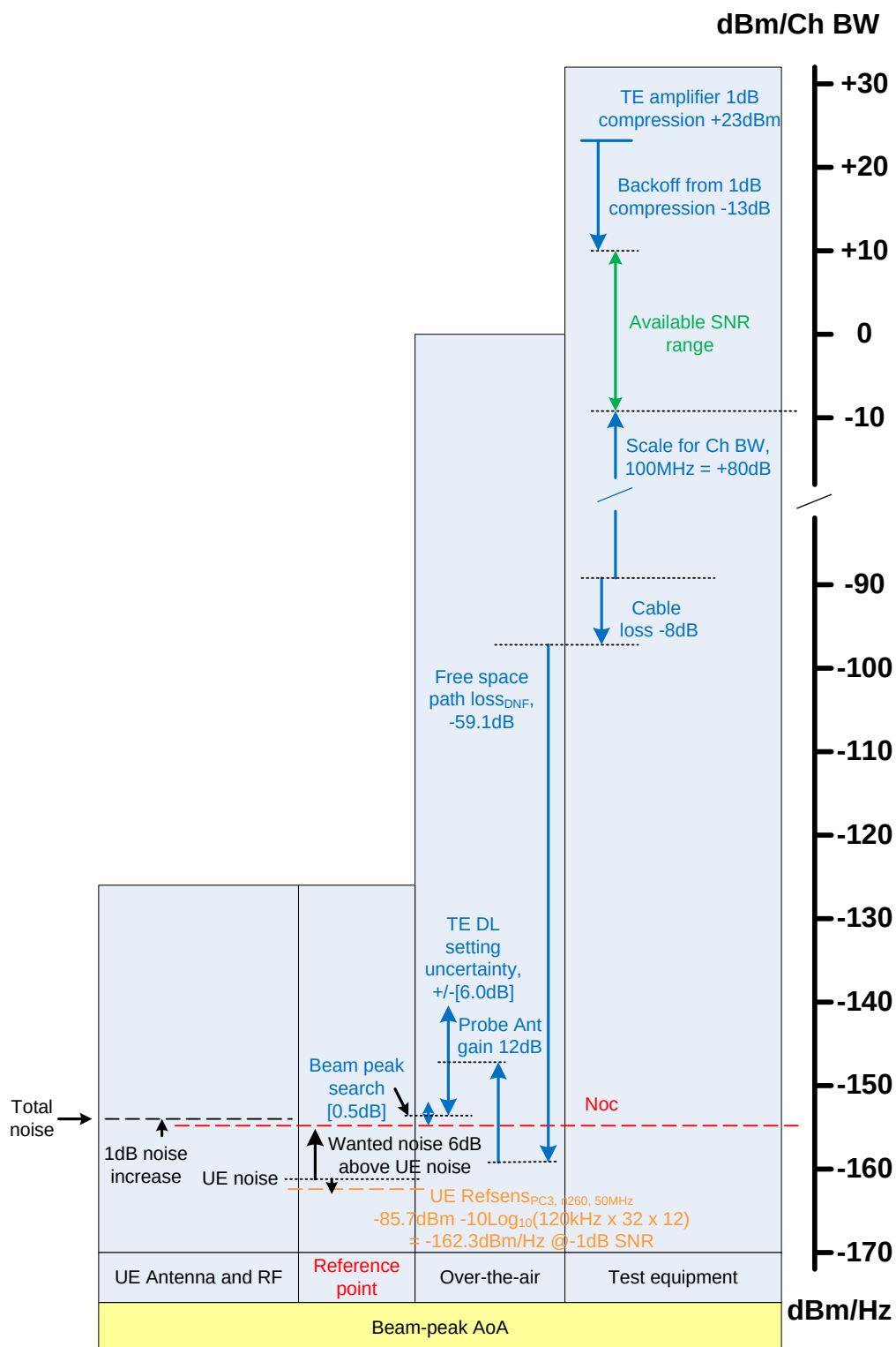
Figure B.3.1.5.4-1: Estimation of single band UE SNR range for Direct near field (DNF)
