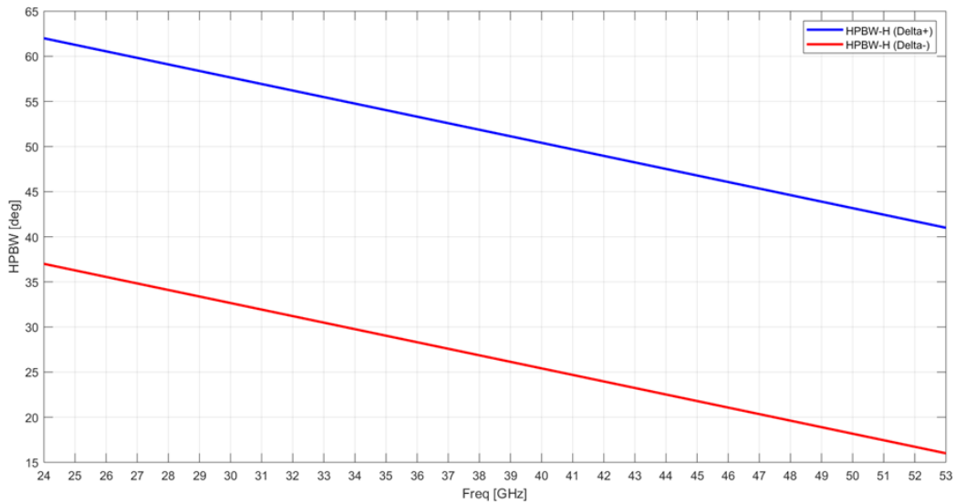
Figure D.2.1-3: 2xHPBW-H mask
