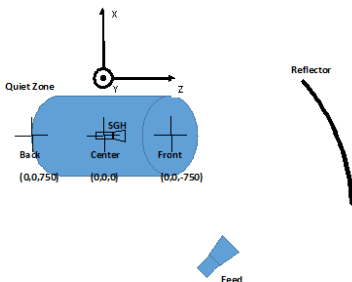
Figure E.3-2: CATR- QZ ripple test (field distribution) set up
