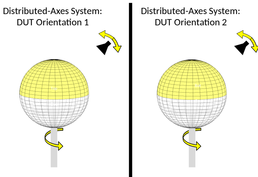
Figure C.3-1: DUT re-positioning for an example of distributed-axes system
