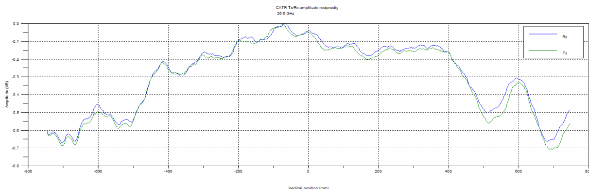
Figure E.3-3: CATR- Amplitude Reciprocity (Vertical cut)
