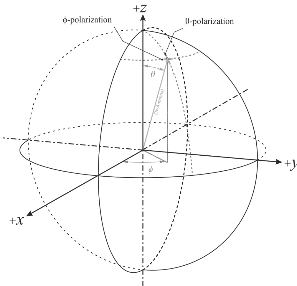
Figure C.1-1: Reference coordinate system
