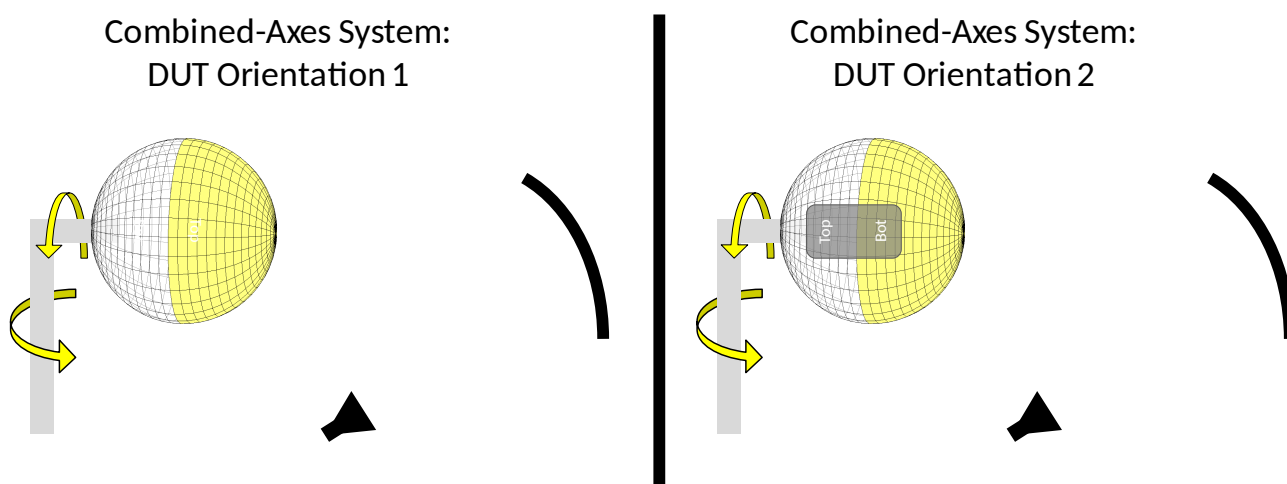
Figure C.3-2: DUT re-positioning for an example of combined-axes system
