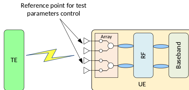
Figure 6.2.1.4.2-1: DL SNR reference point for RRM testing methodology
