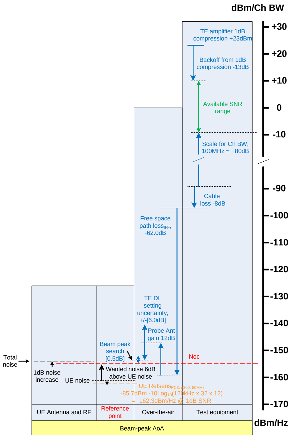
Figure B.3.3.5.4-1: Estimation of single band UE SNR range for Indirect far field (IFF)
