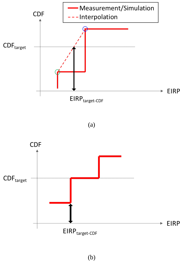
Figure G.3.4-2: Illustration of CDF scenarios, a) CDF target is not met with any EIRP value, b) CDF target is met with one or more EIRP values.
