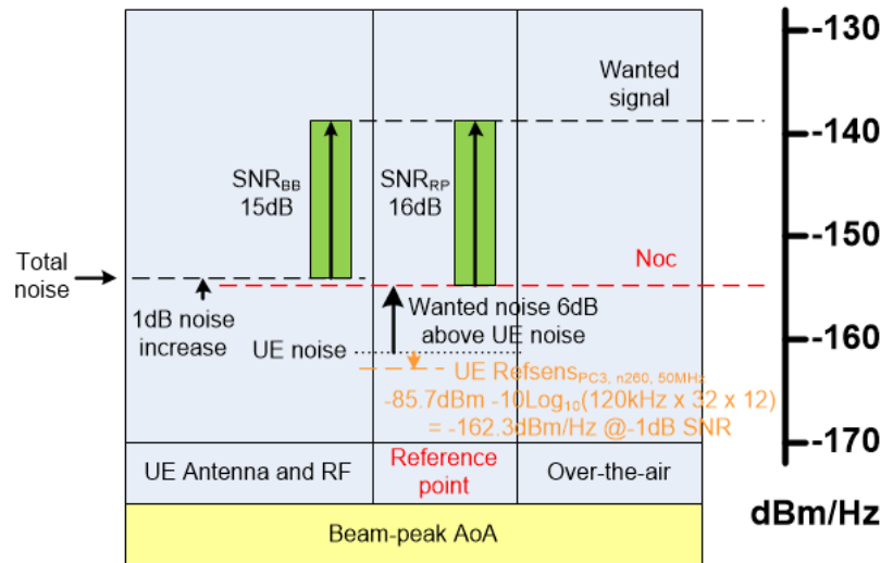
Figure 6.2.1.4.3-1: Reference point SNR_{RP} and Baseband SNR_{BB}
