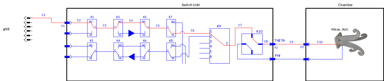
Figure B.1.1.4.4-3: Block Diagram of an EIRP/EIS test case with components from the gNB to the antenna (only portion of switch unit shown)
