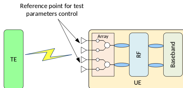
Figure 7.2.1.3-1: DL SNR reference point for UE Demodulation and CSI testing methodology
