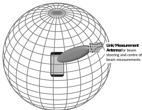
Figure 5.2.1-1: Centre of beam measurement setup of UE RF characteristics
