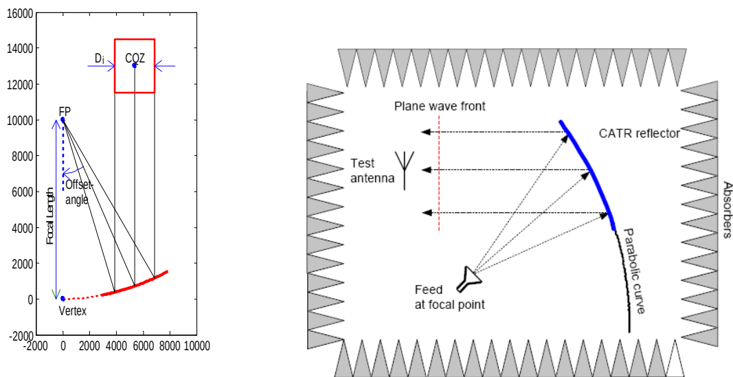
Figure E.1-1: Compact Range – working principle
