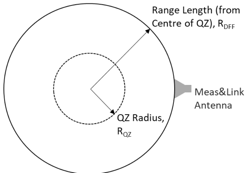
Figure 5.2.1.2-2: Illustration of DFF System for range length definition
