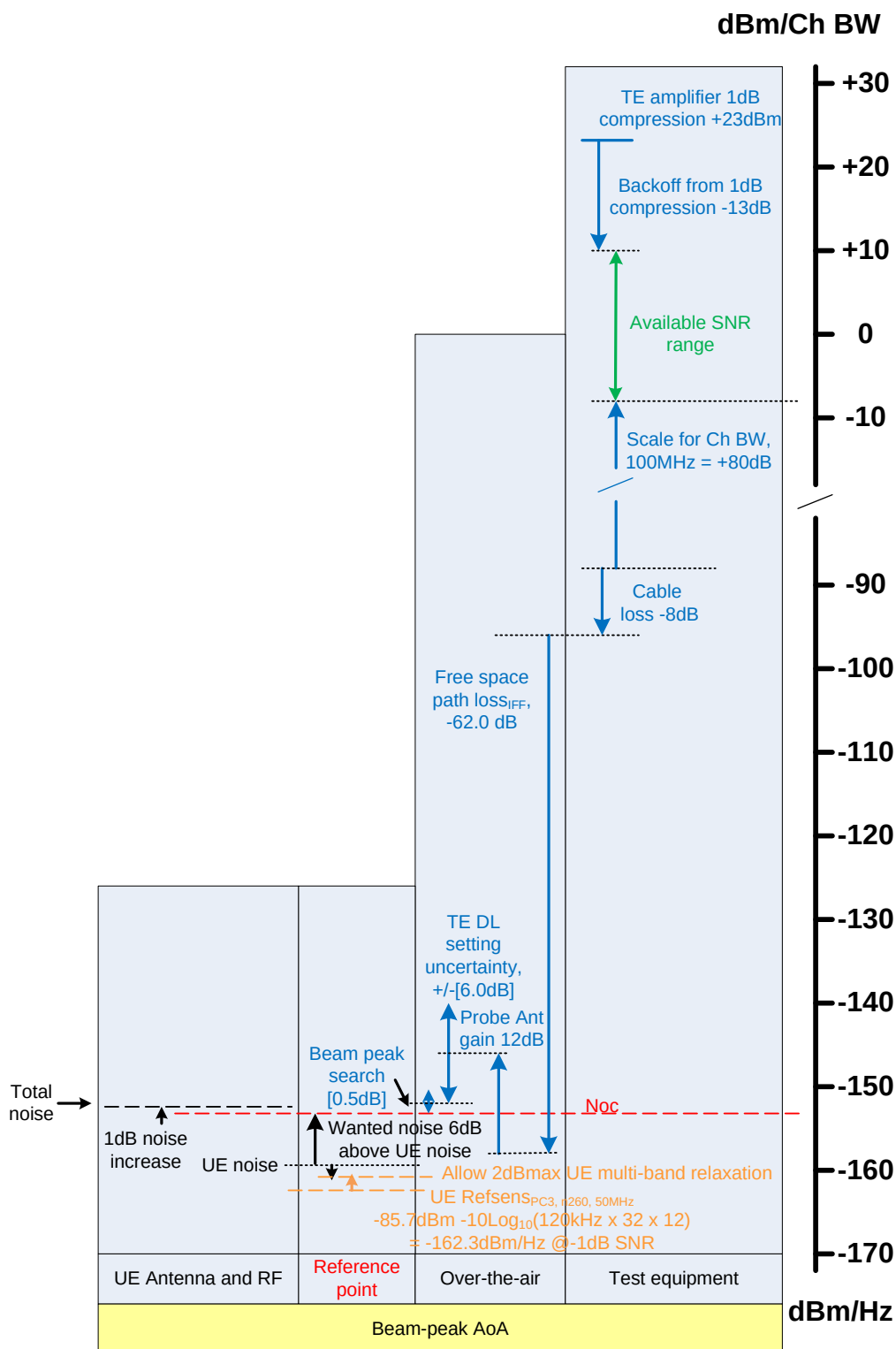
Figure B.2.2.5.4-1: Estimation of multi band UE SNR range for Indirect far field (IFF), fine beam, Rx Beam peak direction
