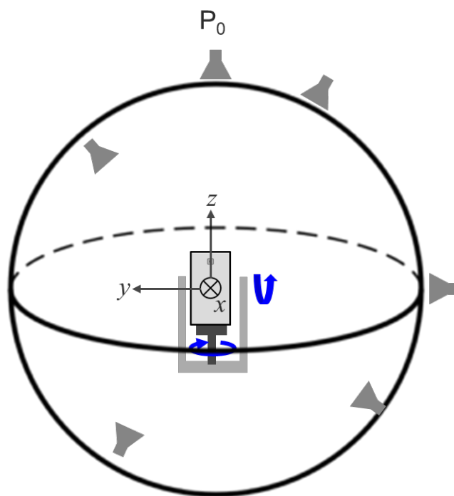
Figure 6.2.1.1-1: Baseline measurement setup of RRM characteristics
