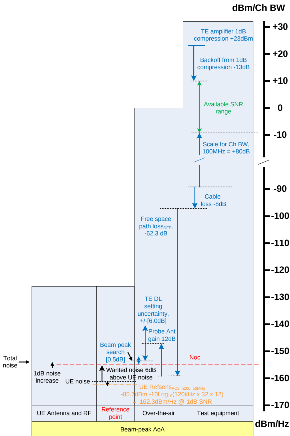
Figure B.3.2.5.4-1: Estimation of single band UE SNR range for Direct far field (DFF)
