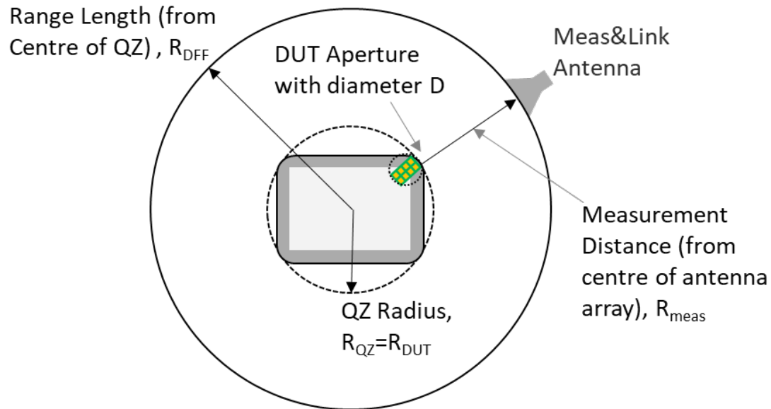
Figure 5.2.1.2-3: Illustration of DFF System for minimum range length definition
