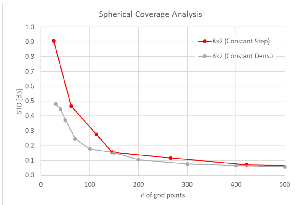
Figure G.3.3.1.1-3: Comparison of the standard deviation of \text{EIRP}_{50\% \text{CDF}} for the 8x2 antenna with the beam peak always placed on a grid point.
