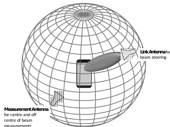
Figure 5.2.1.1-1: DFF measurement setup of UE RF characteristics
