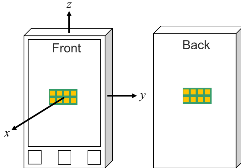
Figure G.3.1-1: Illustration of the two antenna arrays integrated in the UE.
