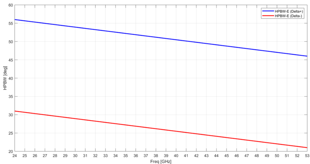
Figure D.2.1-2: 2xHPBW-E mask
