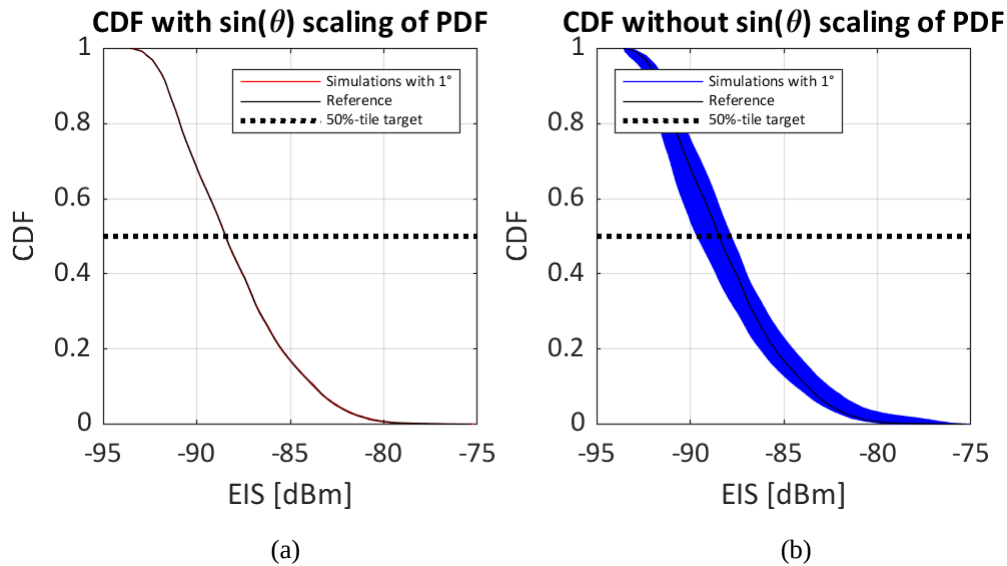
Figure G.3.3.2-1: Sample CDF Analyses for a very fine 1^\circ constant step size measurement grid. a) with the \sin(\theta) scaling of the PDF and b) without the \theta dependent scaling.
