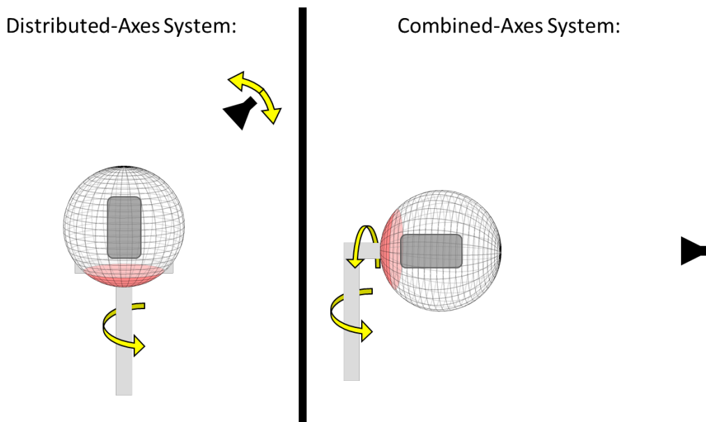
Figure G.1.5-1: Illustration of areas around the pole that either cannot be reached by the measurement antenna or are blocked by the positioner.
