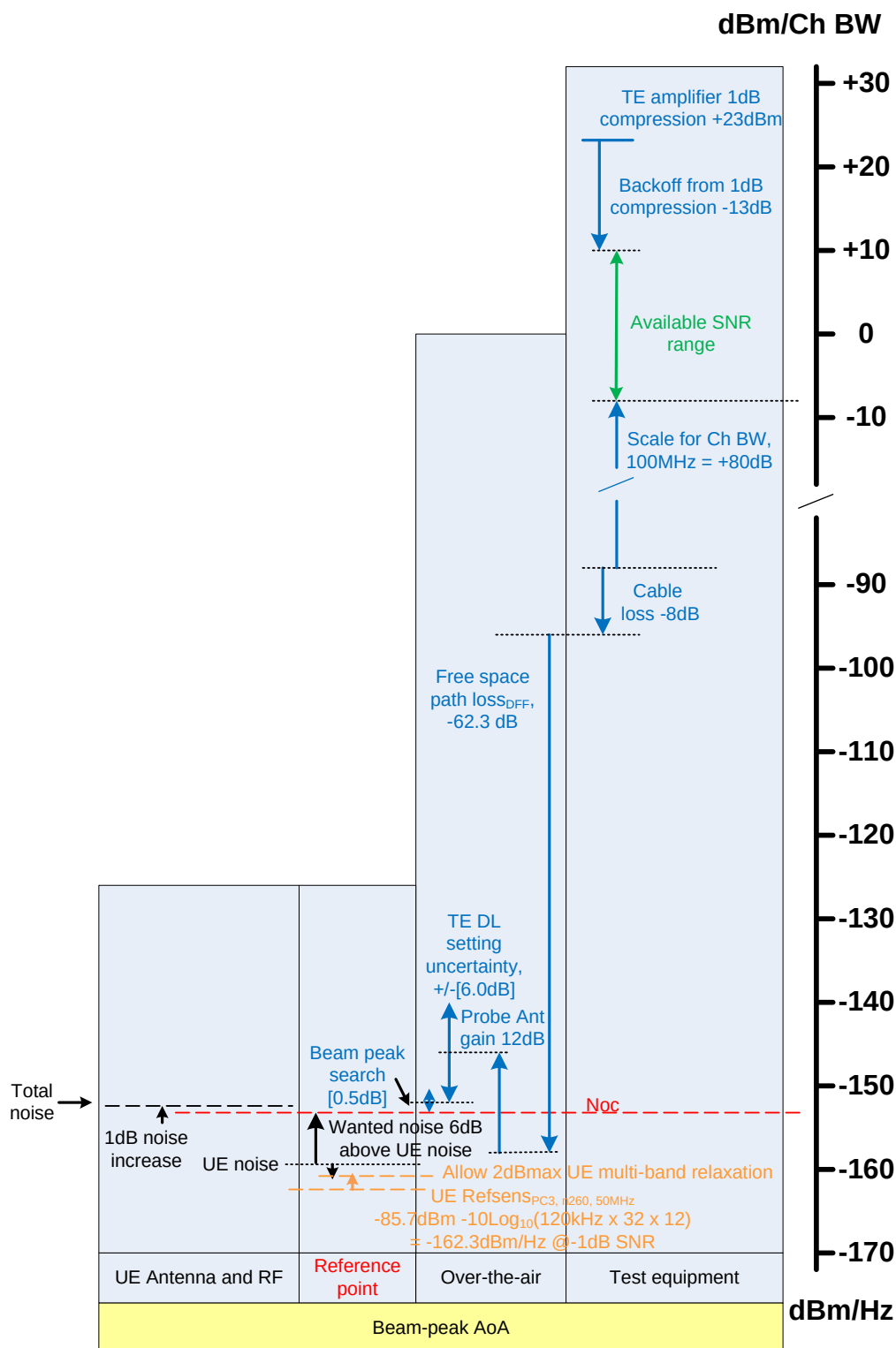
Figure B.2.1.5.4-1: Estimation of multi band UE SNR range for Direct far field (DFF), fine beam, Rx Beam peak direction
