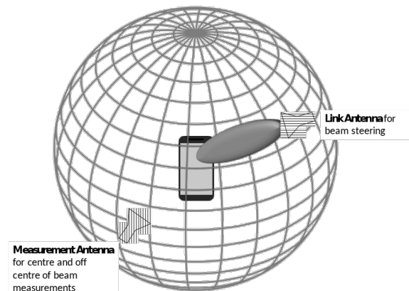
Figure 5.2.1.1-1: DFF measurement setup of UE RF characteristics
