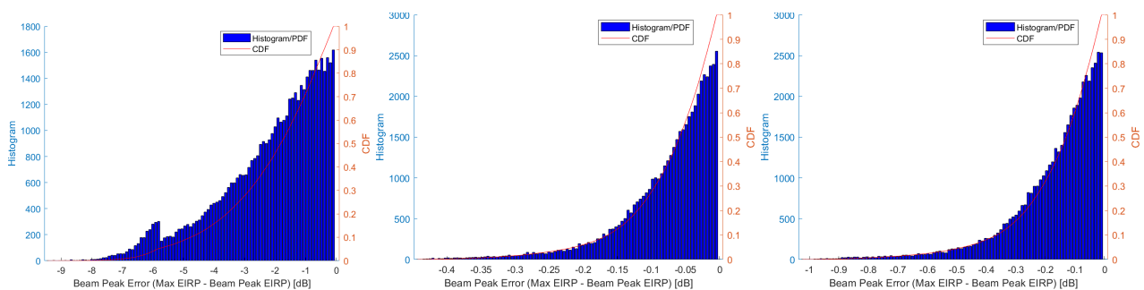
Figure G.2.3-1: Histogram of maximum beam peak errors for sample constant-step size measurement grids (left: 2.5°, middle: 5°, right: 7.5° step size)
