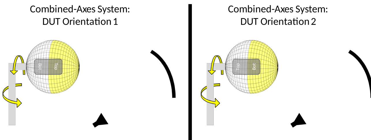
Figure C.3-2: DUT re-positioning for an example of combined-axes system
