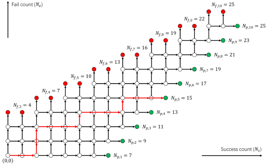
Figure G.5.1-1: Visualization of early decision statistical testing process. In this example, the TE verdicts that the DUT passes the test after executing 15 iterations of test procedure loop. The results of these 15 iterations are “s”, “f”, “f”, “s”, “s”, “s”, “f”, “s”, “s”, “s”, “f”, “s”, “s” and “s” in order (“s” = “success” and “f” = “fail”)
