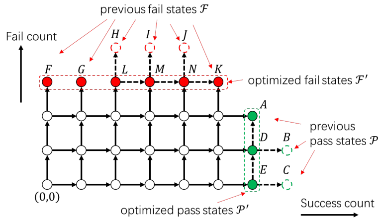
Figure G.5.2-5: Demonstration of step 3 ( n_e doesn't exist).
