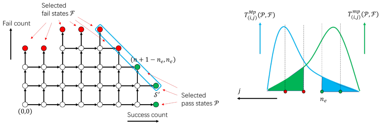
Figure G.5.2-3: Demonstration of step 3 ( n_e exists)
