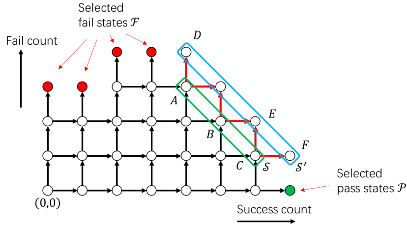
Figure G.5.2-2: Demonstration of step 2
