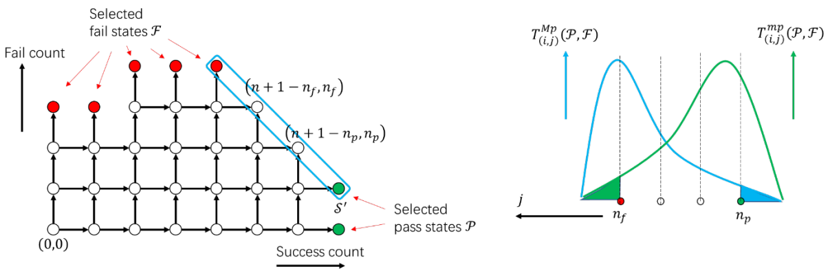
Figure G.5.2-4: Demonstration of step 3 ( n_e doesn't exist)
