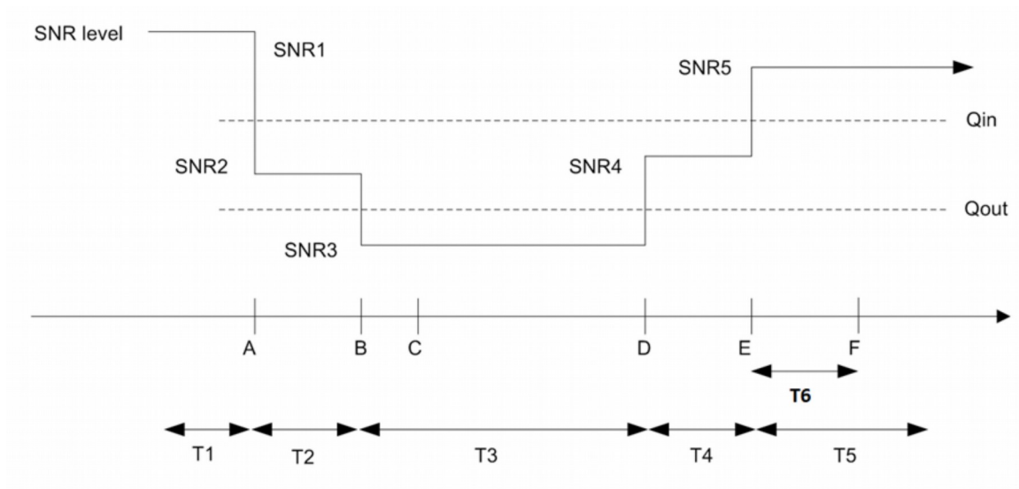
Figure 4.5.1.6.4-1: SNR variation for In-sync testing
