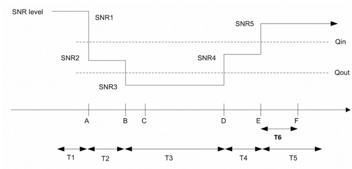
Figure 4.5.1.8.4-1: SNR variation for In-sync testing
