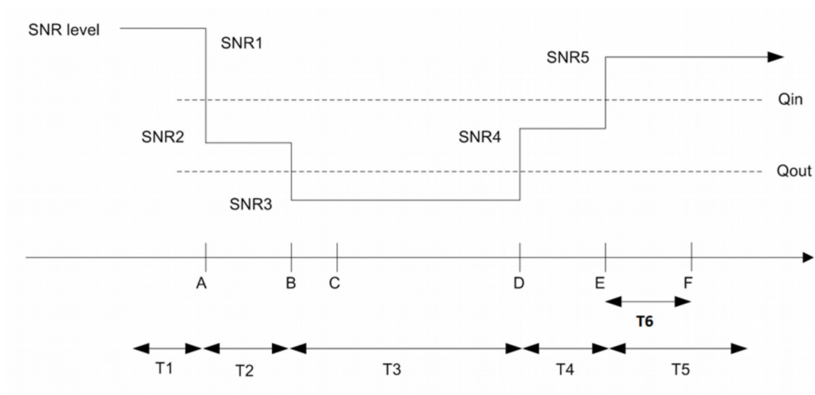
Figure 6.5.1.8.4-1: SNR variation for In-sync testing
