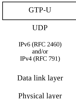
Figure 5.1: Transport network layer for data streams over F1
