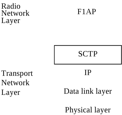
Figure 4.1-1: F1-C signalling bearer protocol stack
