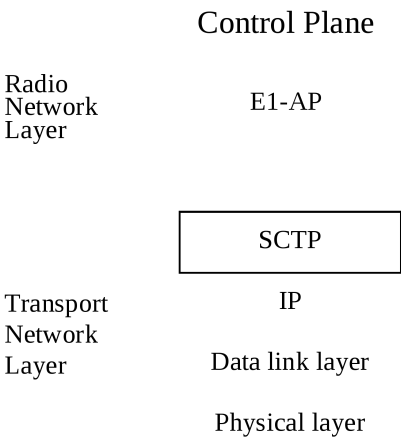
Figure 7.1-1: Interface protocol structure for E1
