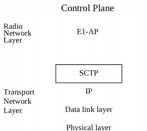
Figure 7.1-1: Interface protocol structure for E1
