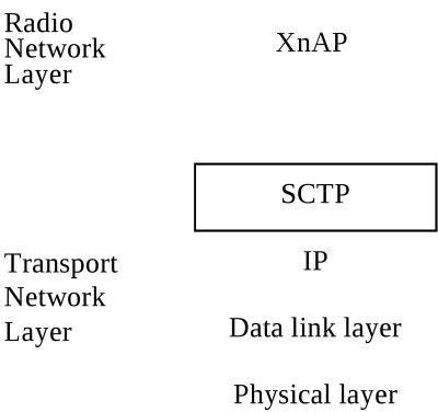
Figure 4.1-1: Xn-C signalling bearer protocol stack
