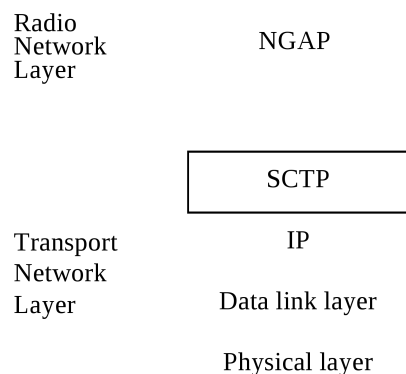
Figure 4.1-1: NG-C signalling bearer protocol stack
