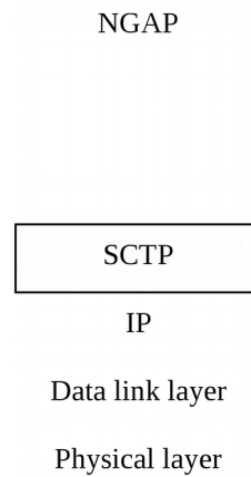
Figure 7.1-1: NG Interface Control Plane
