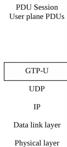
Figure 7.2-1: NG-U protocol structure
