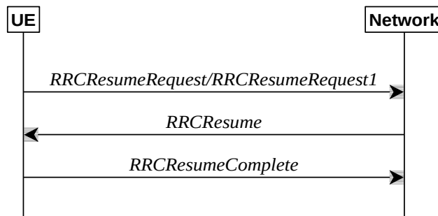
Figure 5.3.13.1-1: RRC connection resume, successful
