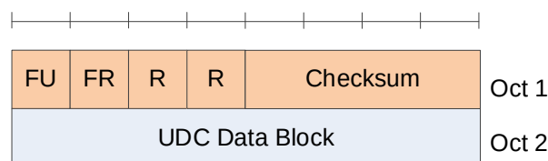
Figure B.2.1-1: UDC header and UDC data block format
