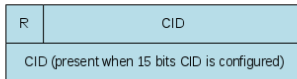
Figure A.2.1.2-1: EHC feedback packet format
