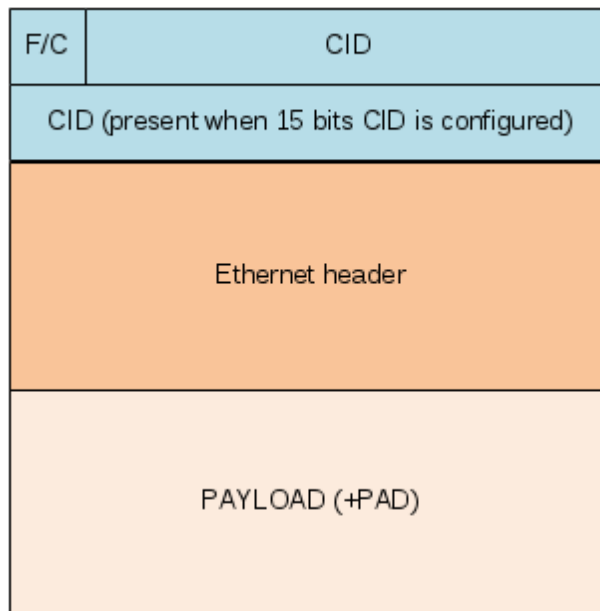
Figure A.2.1.1-1: EHC Full Header packet format
