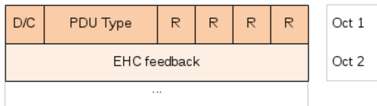
Figure 6.2.3.3-1: PDCP Control PDU format for EHC feedback
