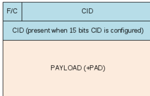
Figure A.2.1.1-2: EHC Compressed Header packet format
