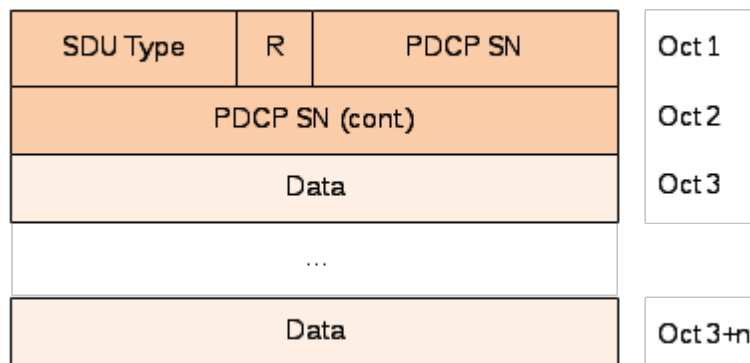
Figure 6.2.2.4-1: PDCP Data PDU format for sidelink DRBs for groupcast and broadcast and for the sidelink SRB0
