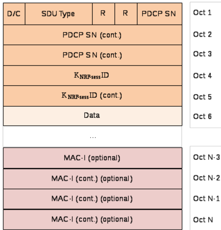
Figure 6.2.2.7-1: PDCP Data PDU format for sidelink DRBs for unicast with 18 bits PDCP SN
