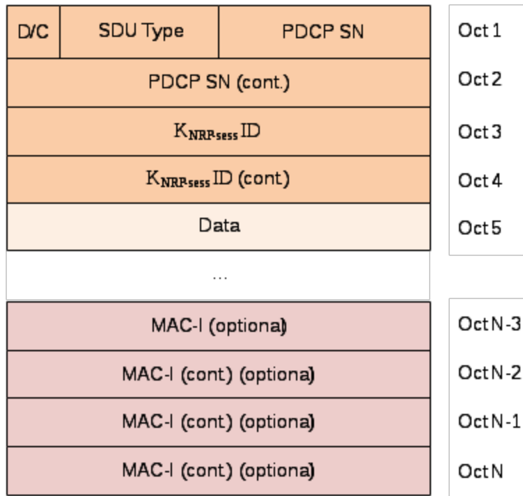
Figure 6.2.2.6-1: PDCP Data PDU format for sidelink DRBs for unicast with 12 bits PDCP SN
