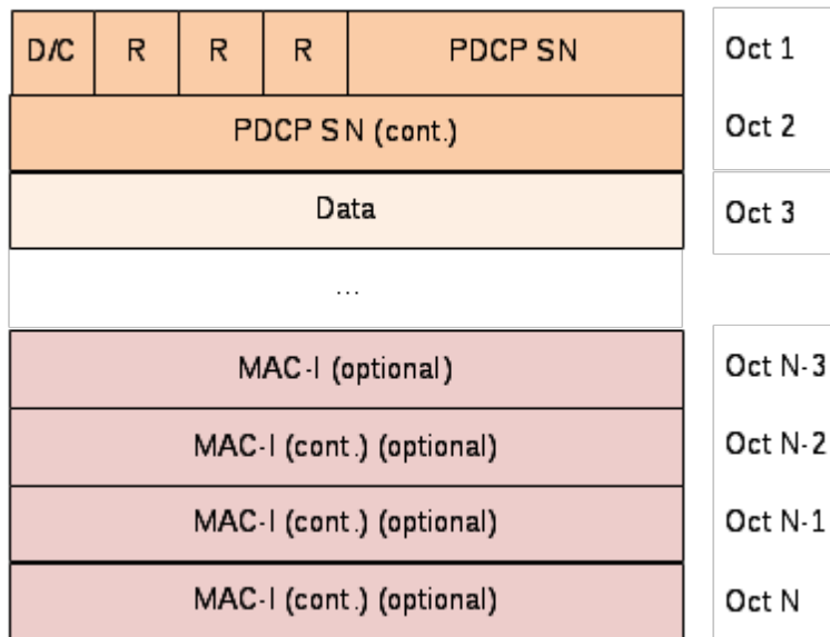
Figure 6.2.2.2-1: PDCP Data PDU format with 12 bits PDCP SN
