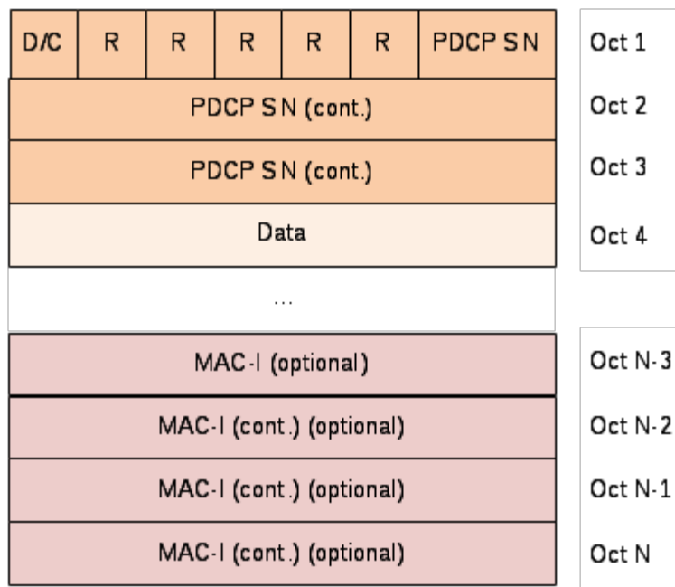
Figure 6.2.2.3-1: PDCP Data PDU format for DRBs with 18 bits PDCP SN
