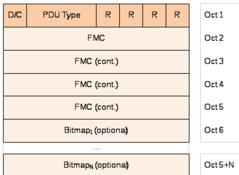
Figure 6.2.3.1-1: PDCP Control PDU format for PDCP status report
