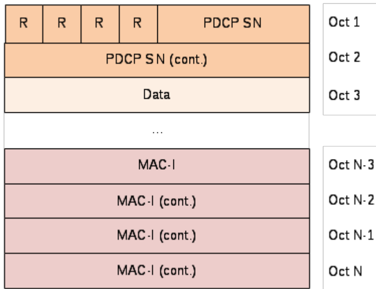
Figure 6.2.2.1-1: PDCP Data PDU format for SRBs
