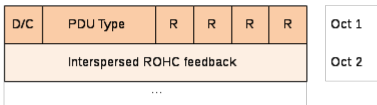
Figure 6.2.3.2-1: PDCP Control PDU format for interspersed ROHC feedback
