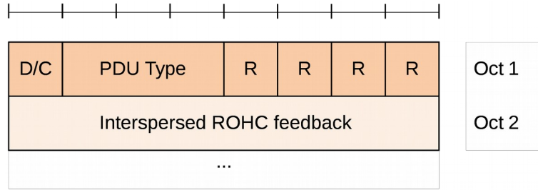
Figure 6.2.3.2-1: PDCP Control PDU format for interspersed ROHC feedback
