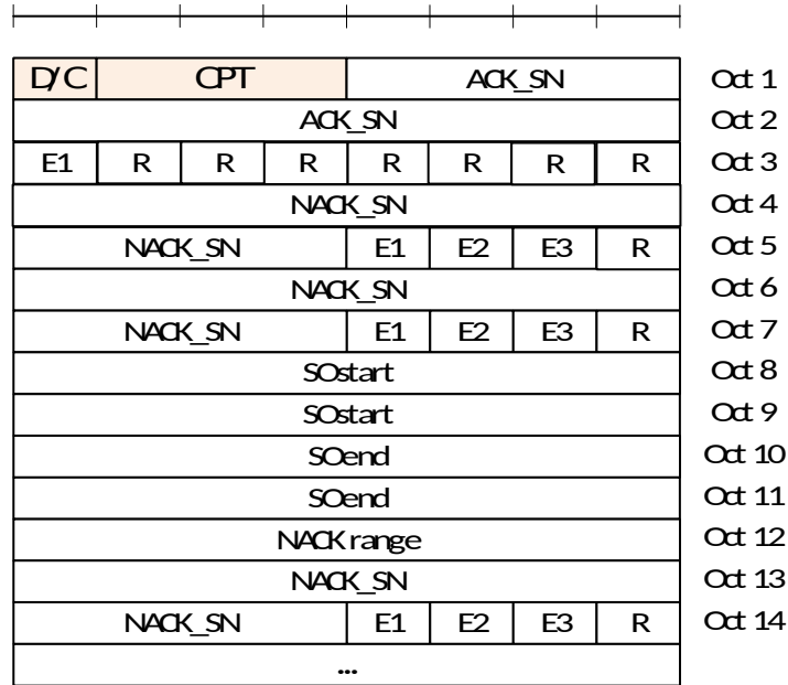
Figure 6.2.2.5-1: STATUS PDU with 12 bit SN
