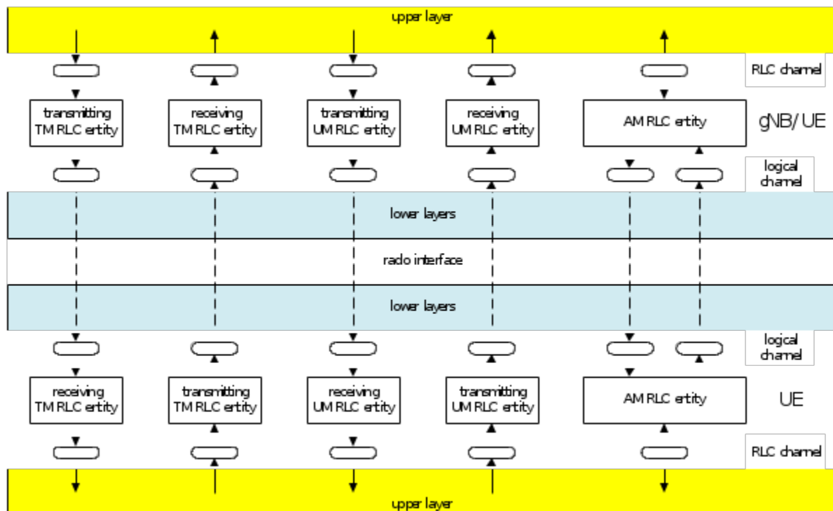
Figure 4.2.1-1 illustrates the overview model of the RLC sub layer.
