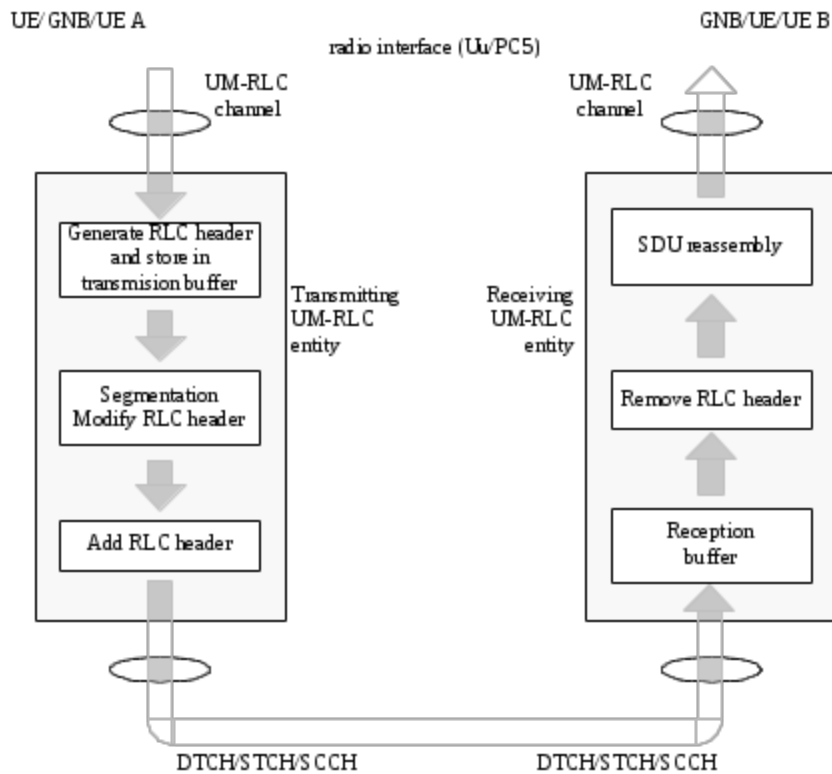
Figure 4.2.1.2.1-1: Model of two unacknowledged mode peer entities
