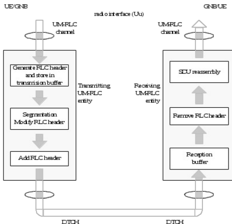
Figure 4.2.1.2.1-1: Model of two unacknowledged mode peer entities
