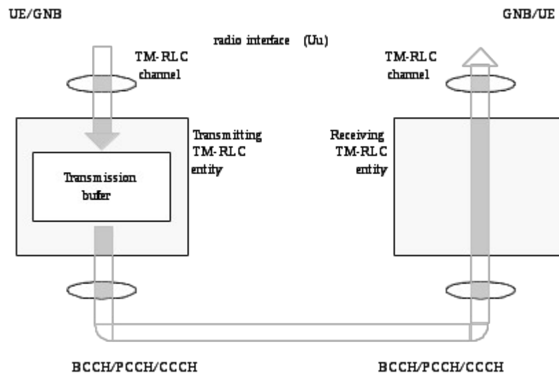
Figure 4.2.1.1.1-1: Model of two transparent mode peer entities
