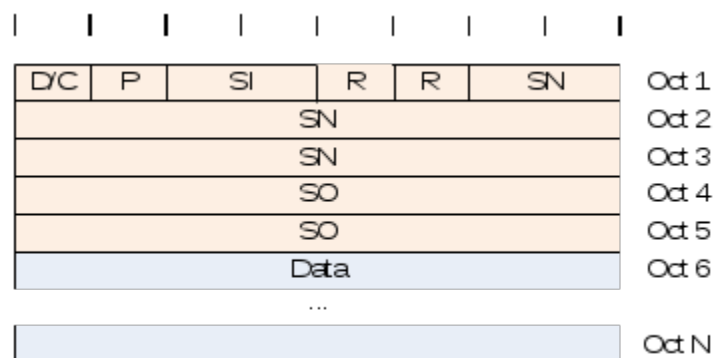
Figure 6.2.2.4-3: AMD PDU with 12 bit SN with SO
