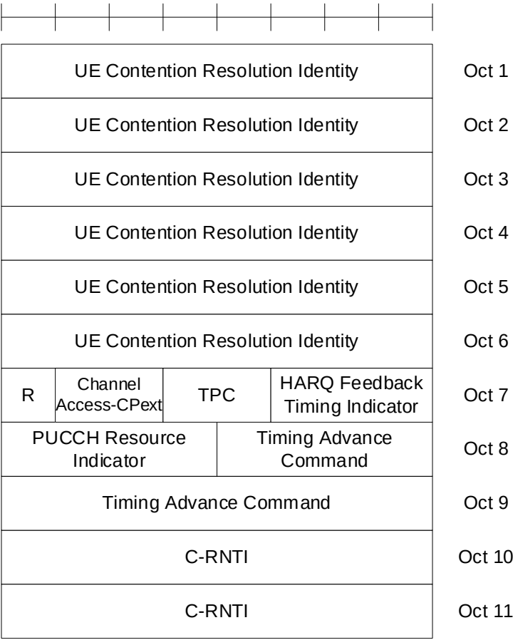
Figure 6.2.3a-2: successRAR
