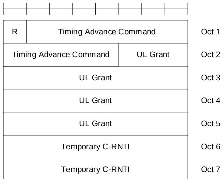
Figure 6.2.3a-1: fallbackRAR
