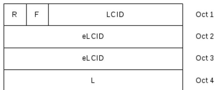
Figure 6.1.2-1: R/F/LCID/(eLCID)/L MAC subheader with 8-bit L field
