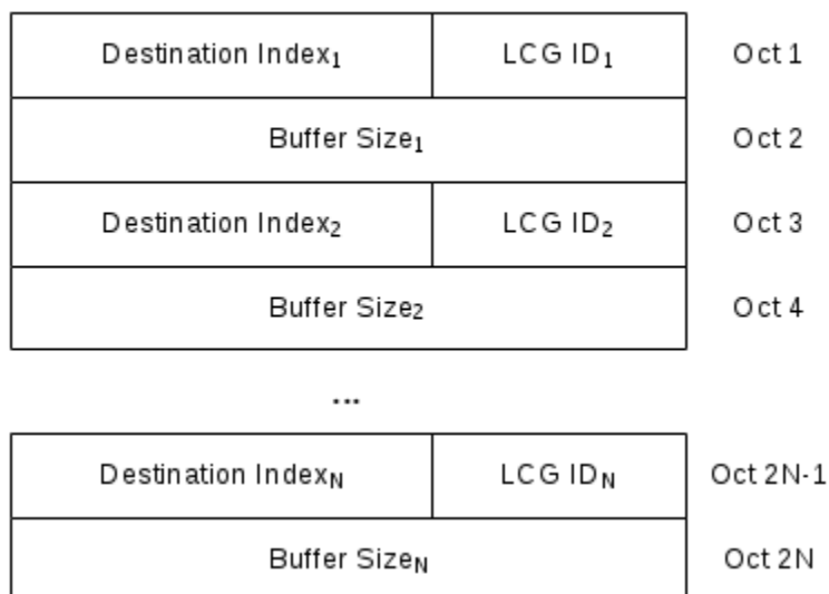
Figure 6.1.3.33-1: SL-BSR and Truncated SL-BSR MAC control element
