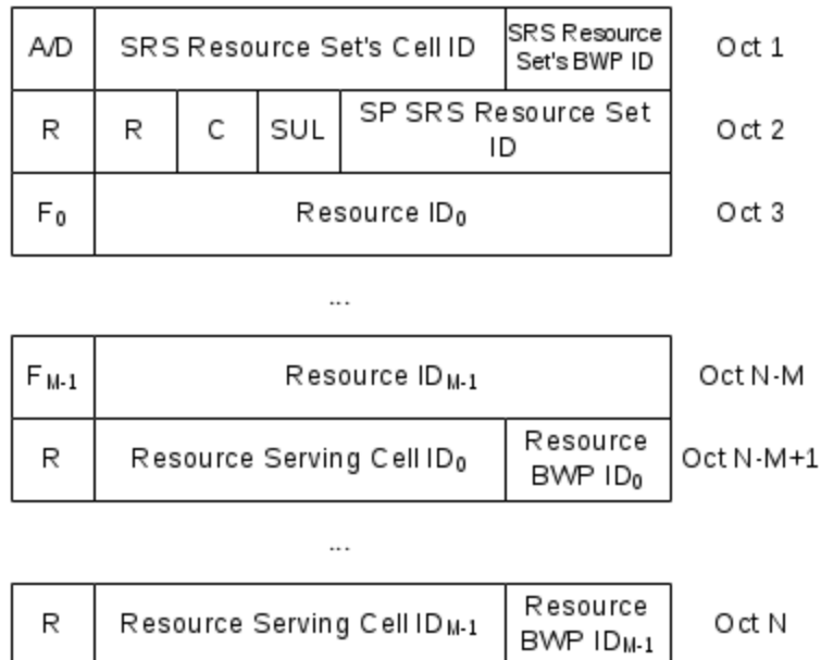
Figure 6.1.3.17-1: SP SRS Activation/Deactivation MAC CE
