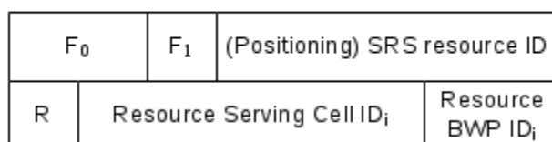
Figure 6.1.3.36-4: Spatial Relation for Resource ID i with SRS
