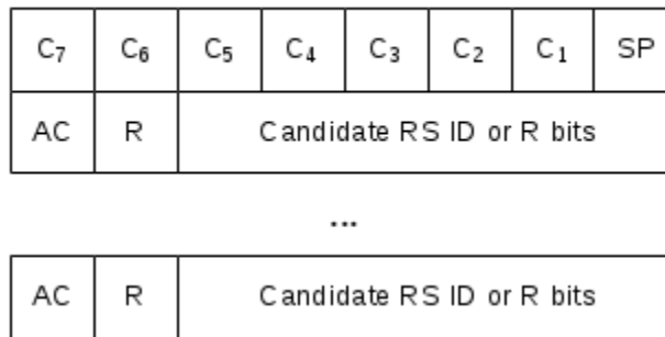
Figure 6.1.3.23-1: BFR and Truncated BFR MAC CE with one octet C i field
