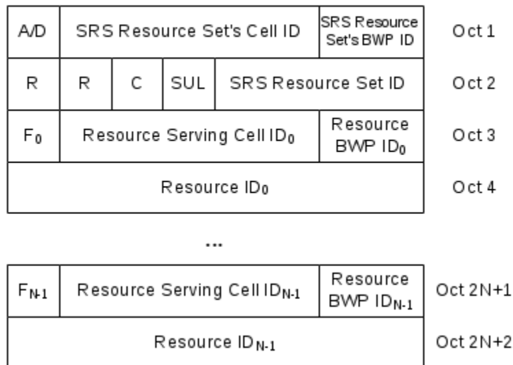
Figure 6.1.3.26-1: Enhanced SP/AP SRS spatial relation Indication MAC CE
