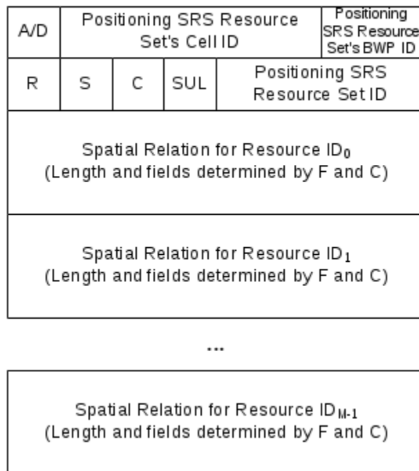
Figure 6.1.3.36-1: SP Positioning SRS Activation/Deactivation MAC CE
