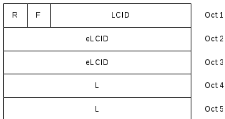
Figure 6.1.2-2: R/F/LCID/(eLCID)/L MAC subheader with 16-bit L field
