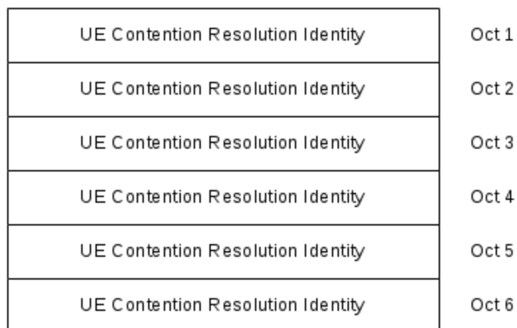
Figure 6.1.3.3-1: UE Contention Resolution Identity MAC CE
