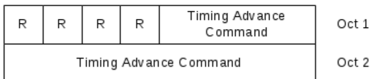
Figure 6.1.3.4a-1: Absolute Timing Advance Command MAC CE
