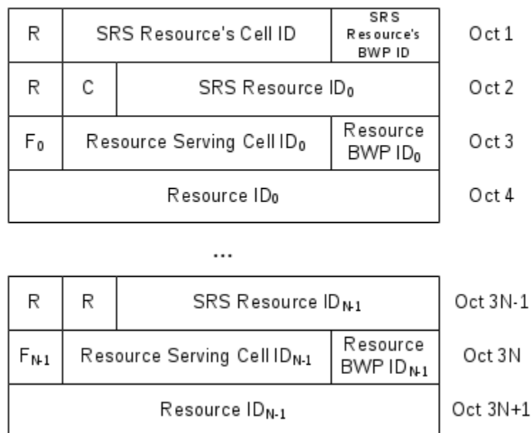
Figure 6.1.3.29-1: Serving Cell set based SRS Spatial Relation Indication MAC CE
