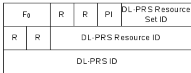
Figure 6.1.3.36-5: Spatial Relation for Resource ID i with DL-PRS
