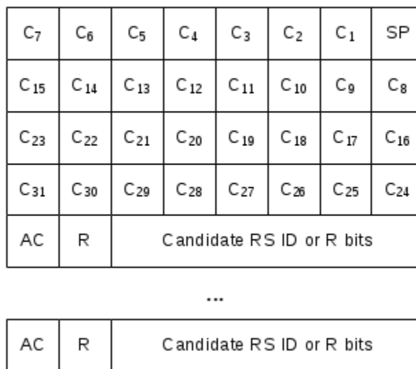
Figure 6.1.3.23-2: BFR and Truncated BFR MAC CE with four octets C i field
