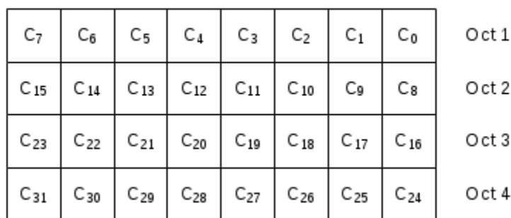
Figure 6.1.3.30-2: LBT failure MAC CE of four octets
