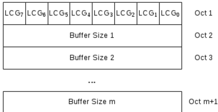
Figure 6.1.3.1-2: Long BSR, Long Truncated BSR, and Pre-emptive BSR MAC CE
