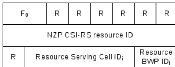
Figure 6.1.3.36-2: Spatial Relation for Resource ID i with NZP CSI-RS
