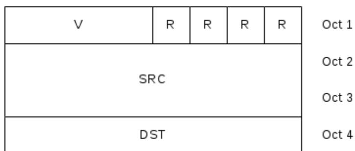
Figure 6.1.6-1: SL-SCH MAC subheader
