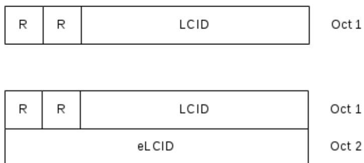
Figure 6.1.2-3: R/LCID/(eLCID) MAC subheader
