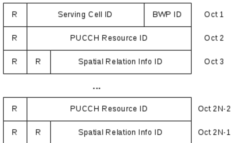
Figure 6.1.3.25-1: Enhanced PUCCH spatial relation Activation/Deactivation MAC CE
