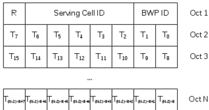
Figure 6.1.3.13-1: Aperiodic CSI Trigger State Subselection MAC CE
