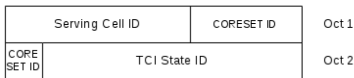
Figure 6.1.3.15-1: TCI State Indication for UE-specific PDCCH MAC CE
