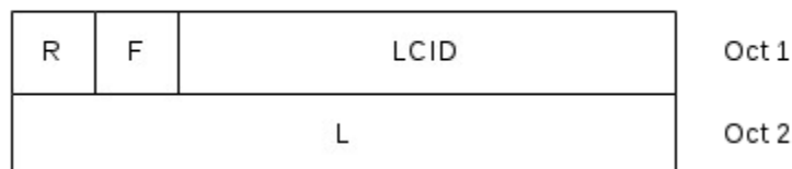
Figure 6.1.2-1: R/F/LCID/L MAC subheader with 8-bit L field
