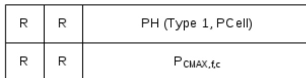
Figure 6.1.3.8-1: Single Entry PHR MAC CE
