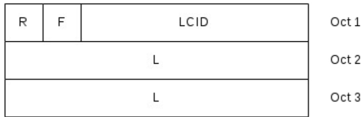
Figure 6.1.2-2: R/F/LCID/L MAC subheader with 16-bit L field
