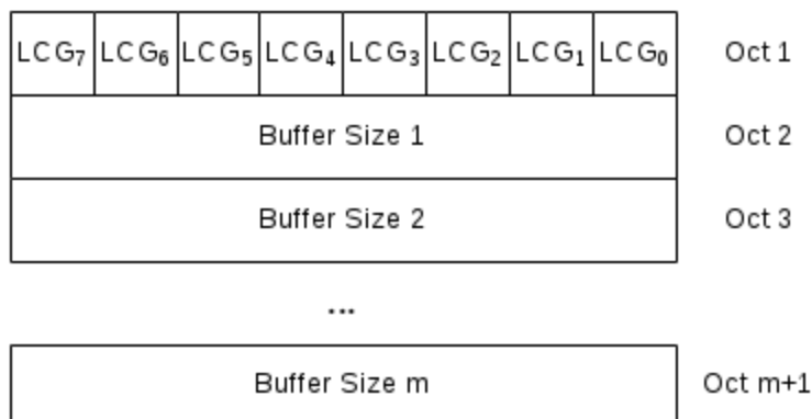
Figure 6.1.3.1-2: Long BSR and Long Truncated BSR MAC CE
