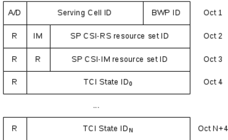
Figure 6.1.3.12-1: SP CSI-RS/CSI-IM Resource Set Activation/Deactivation MAC CE
