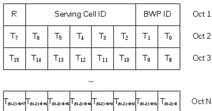
Figure 6.1.3.14-1: TCI States Activation/Deactivation for UE-specific PDSCH MAC CE
