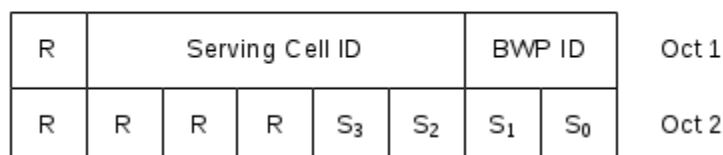
Figure 6.1.3.16-1: SP CSI reporting on PUCCH Activation/Deactivation MAC CE
