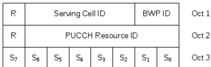
Figure 6.1.3.18-1: PUCCH spatial relation Activation/Deactivation MAC CE
