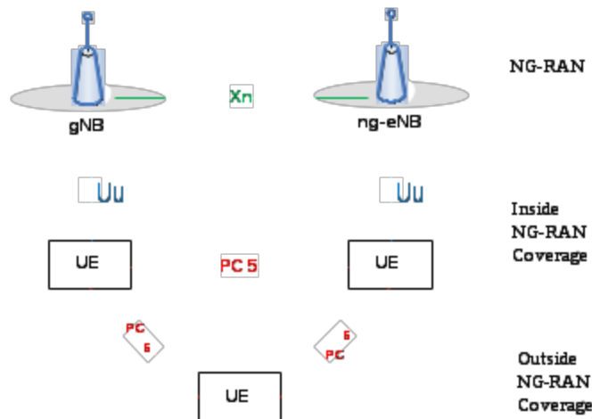
Figure 16.9.1-1: NG-RAN Architecture supporting the PC5 interface
