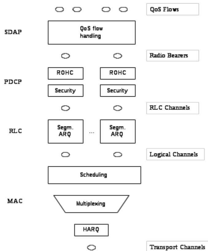
Figure 6.1-2: Uplink Layer 2 Structure
