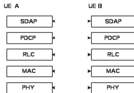
Figure 16.9.2.1-4: User plane protocol stack for STCH.
