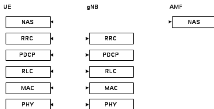
Figure 4.4.2-1: Control Plane Protocol Stack
