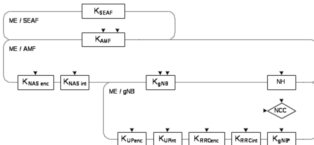
Figure 13.1-1: 5G Key Derivation
