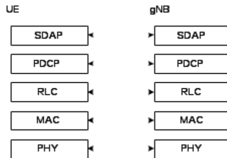
Figure 4.4.1-1: User Plane Protocol Stack
