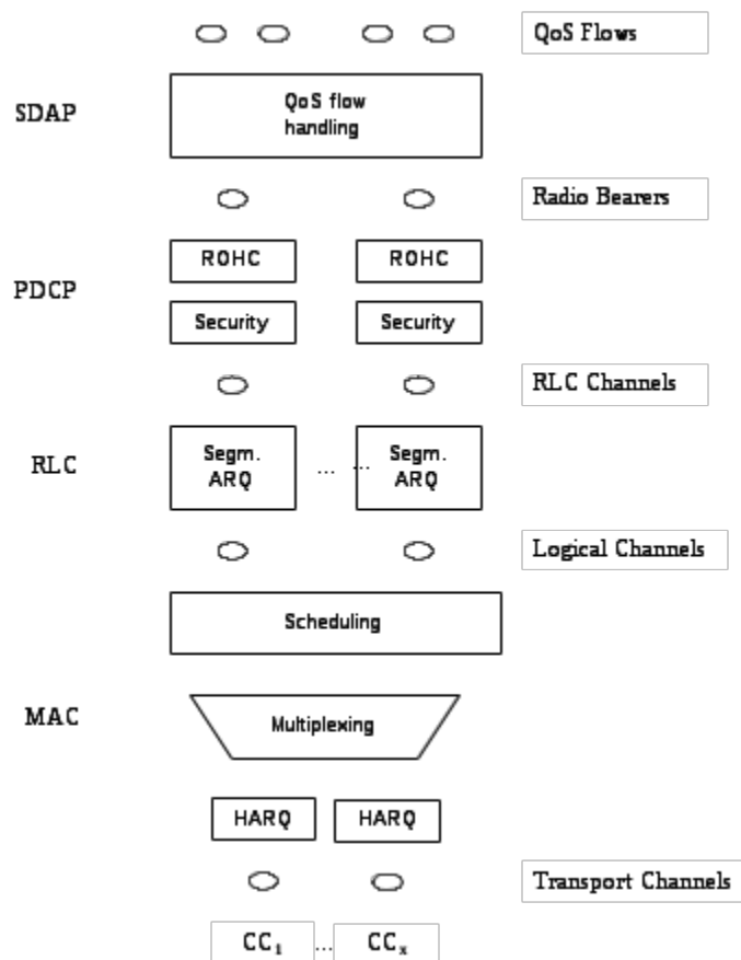
Figure 6.7-2: Layer 2 Structure for UL with CA configured
