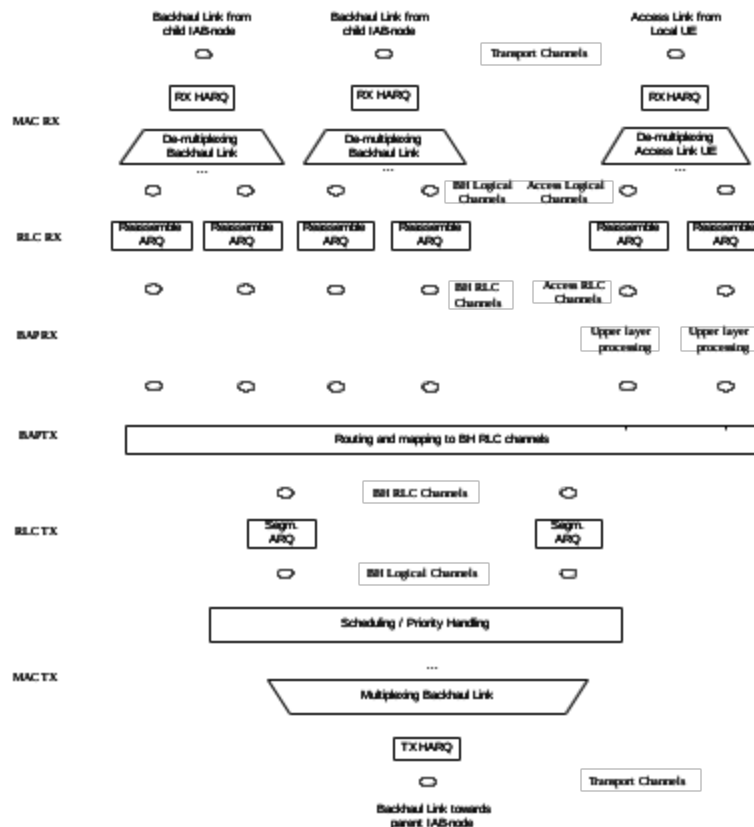
Figure 6.1-5: UL L2-structure at IAB-node
