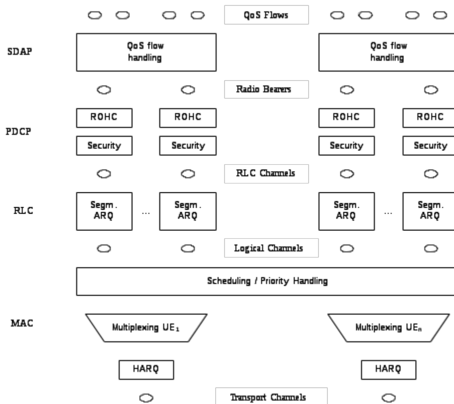
Figure 6.1-1: Downlink Layer 2 Structure
