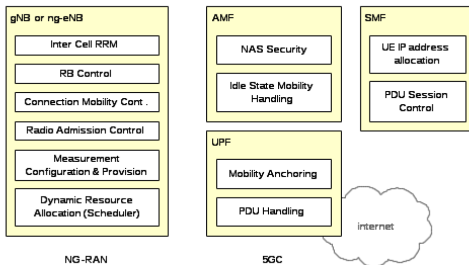
Figure 4.2-1: Functional Split between NG-RAN and 5GC
