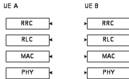
Figure 16.9.2.1-3: Control plane protocol stack for SBCCH.
