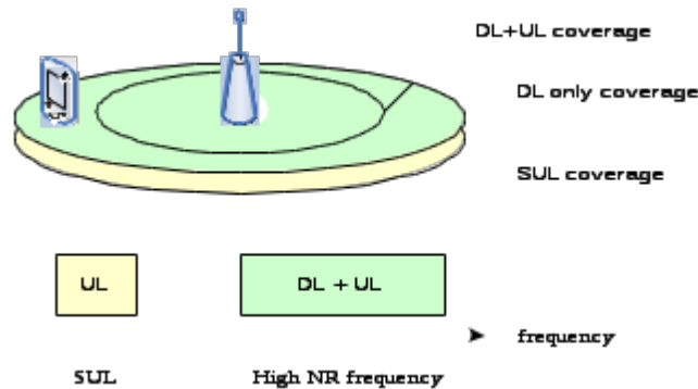
Figure B.1-1: Example of Supplementary Uplink
