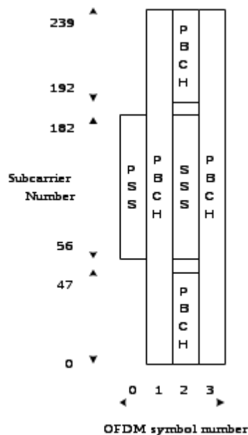
Figure 5.2.4-1: Time-frequency structure of SSB
