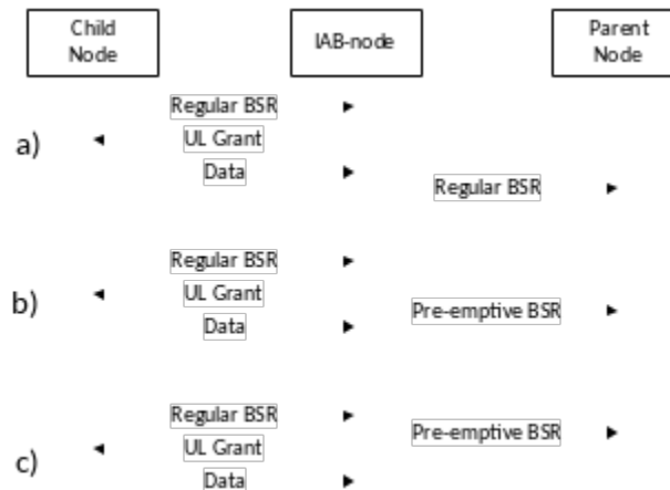
Figure 4.7.3.3-1: Scheduling of BSR in IAB:
