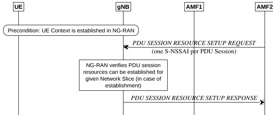
Figure 16.3.4.4-1: Network Slice-aware PDU Session Resource Setup
