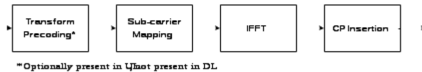
Figure 5.1-1: Transmitter block diagram for CP-OFDM with optional DFT-spreading
