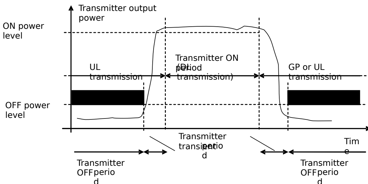
Figure 6.4.2.1-1: Example of relations between transmitter ON period, transmitter OFF period and transmitter transient period
